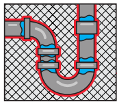
CONSTRUCTION & INSTALL OATEY GREAT BLUE® PIPE JOINT COMPOUND STEEL SINK PIPE AND P-TRAP HERCULES MEGALOC® HERCULES MEGATAPE®
